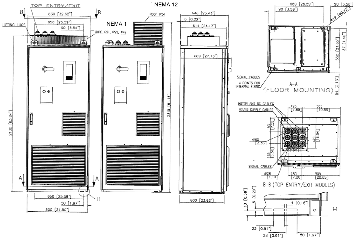
Drive Dimensions
